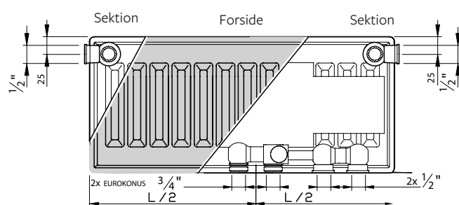
Type 21, 22, 33
