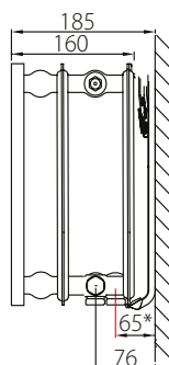
Type 30
