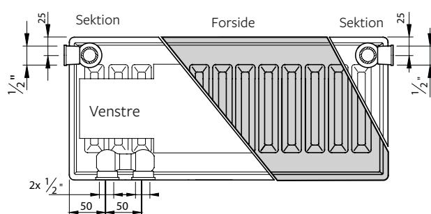
Type 21, 22, 33 - VENSTRE
